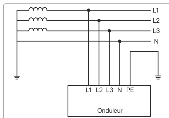
Figure 4-7 TT
