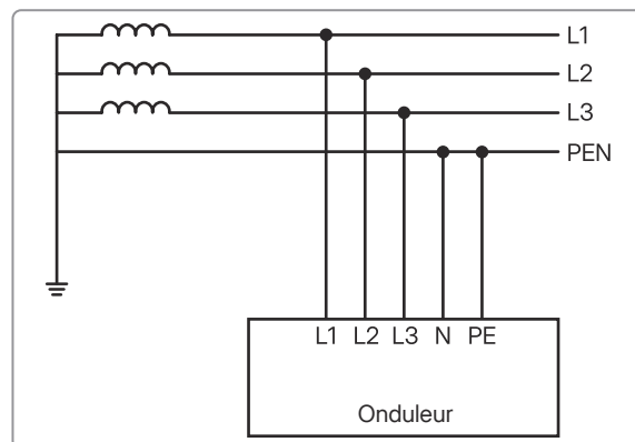
Figure 4-5 TN-C
